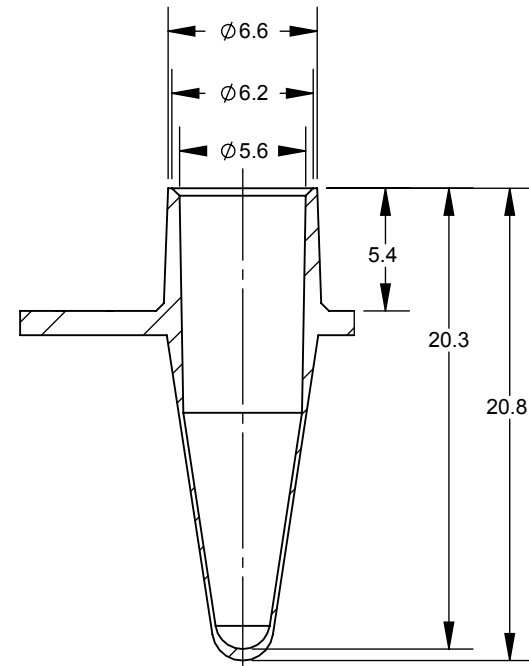
DETAIL B
