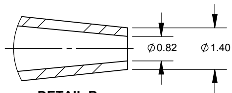
DETAIL B
