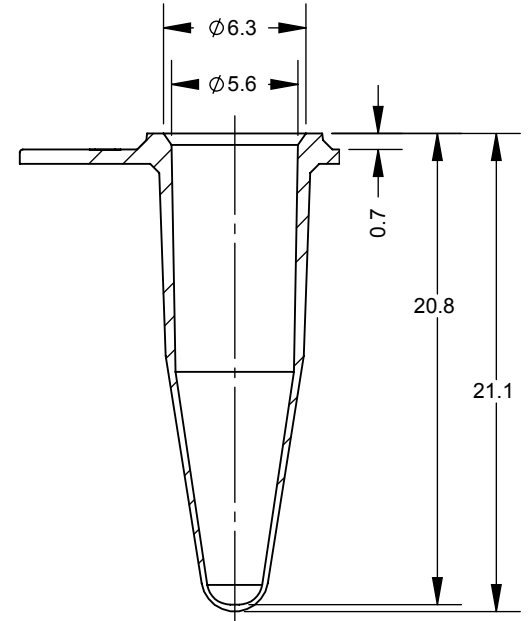
DETAIL B
