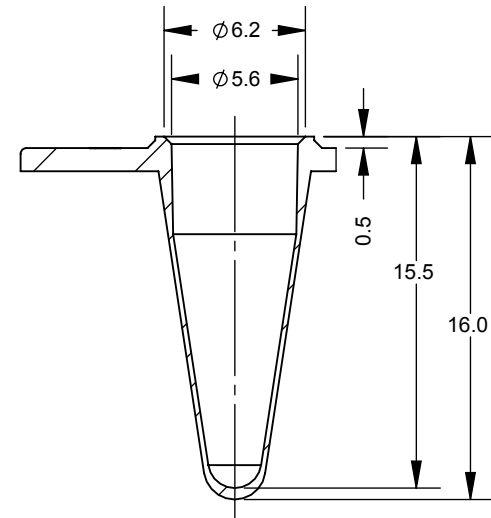
DETAIL B
