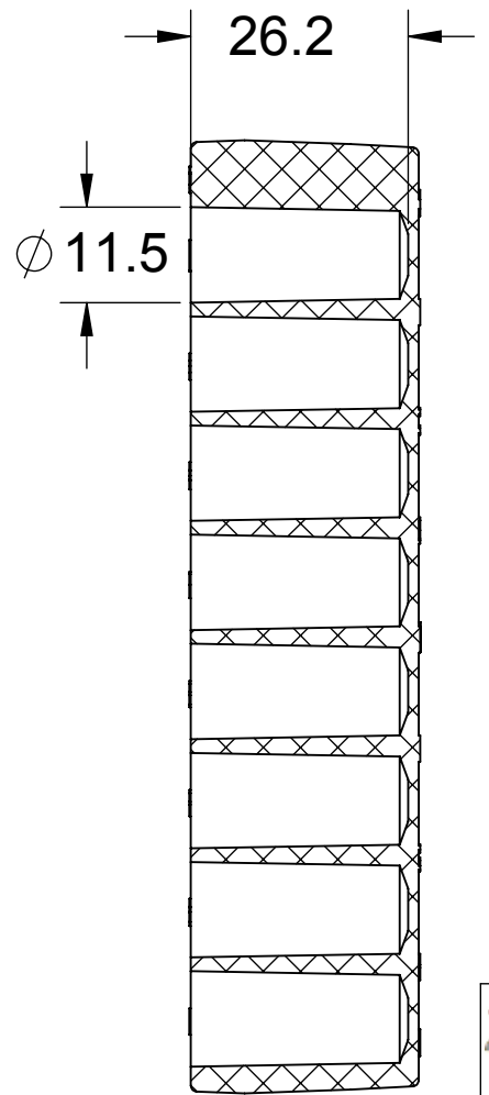
SECTION B-B
