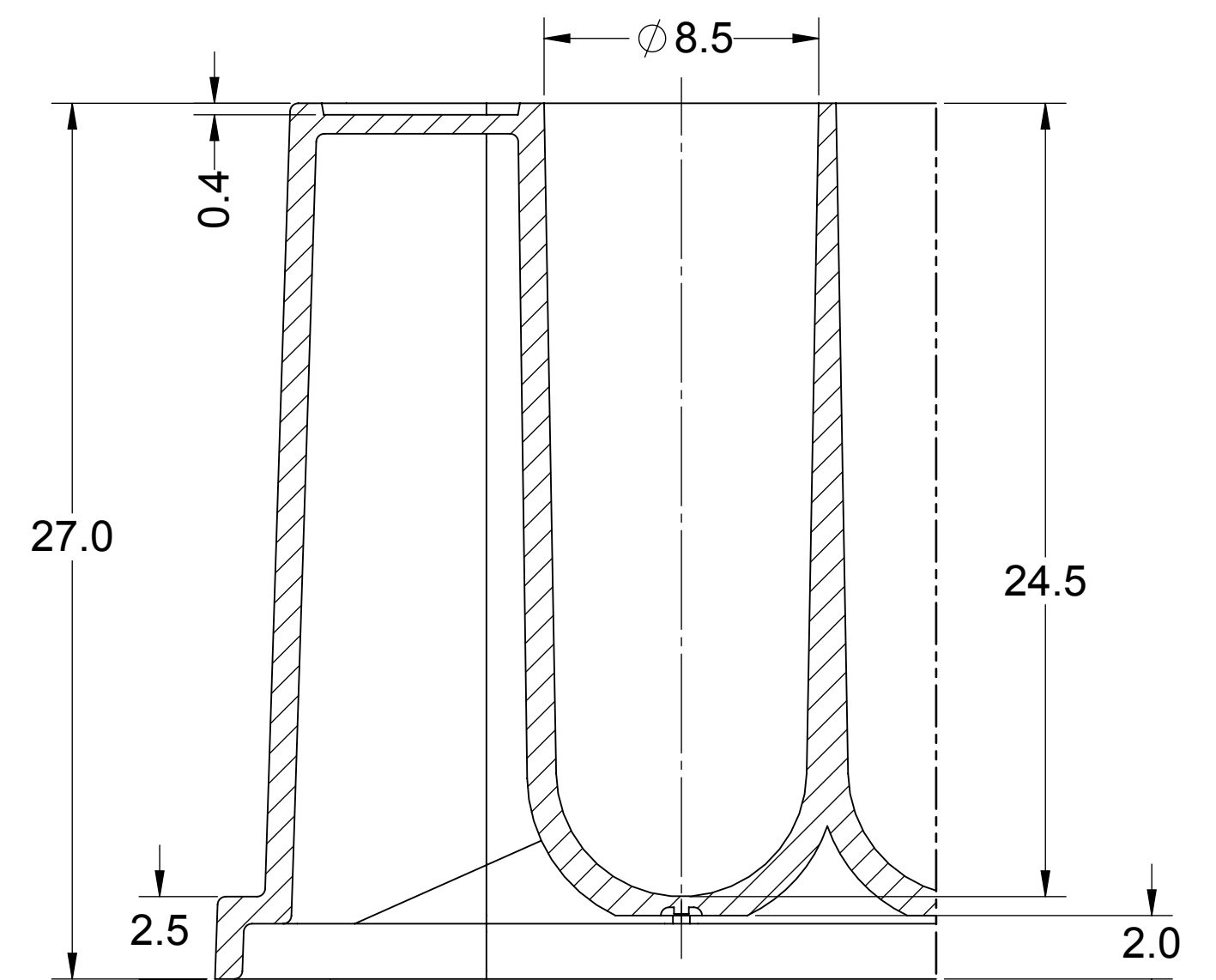
DETAIL B
